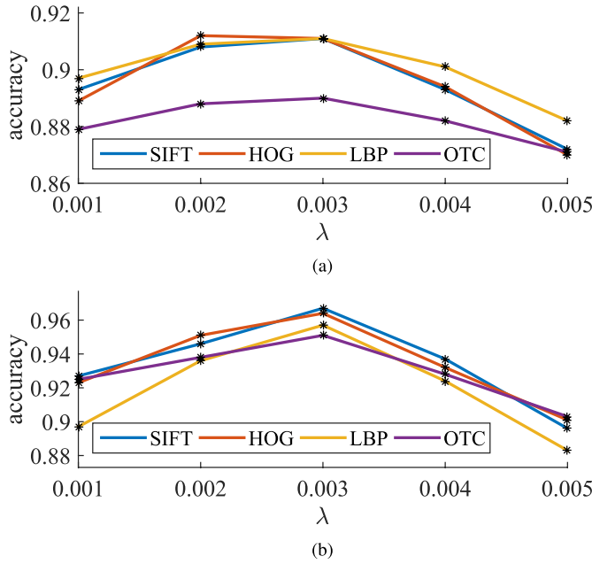
Fig. 12. Average scene classification accuracy for \lambda = 0.001, 0.002, 0.003, 0.004, 0.005 . (a) MSRC dataset. (b) SIFT flow dataset.
