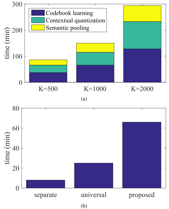
Fig. 14. Computational complexity analysis. (a) time consumption of codebook learning, contextual quantization and semantic pooling in the proposed algorithm ( K = 500, 1000, 2000 ); (b) time consumption of separate codebook learning, universal codebook learning and the proposed multitask codebook learning.
