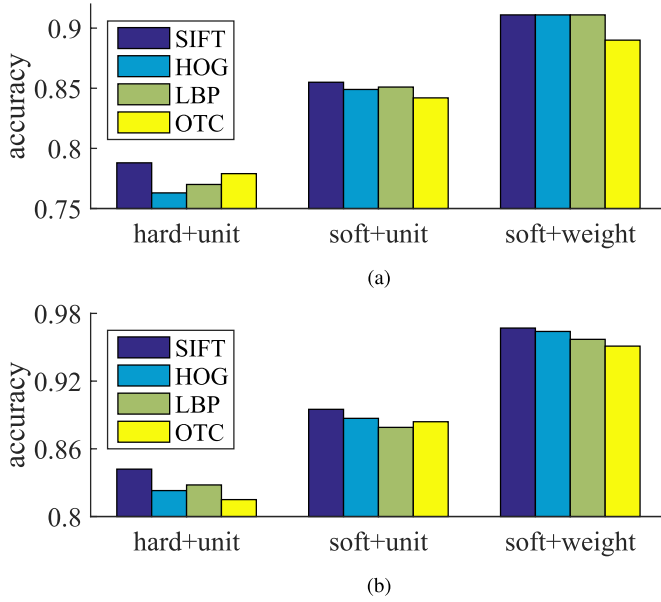
Fig. 10. Average scene classification accuracy of different pooling schemes. (a) MSRC dataset. (b) SIFT flow dataset.
