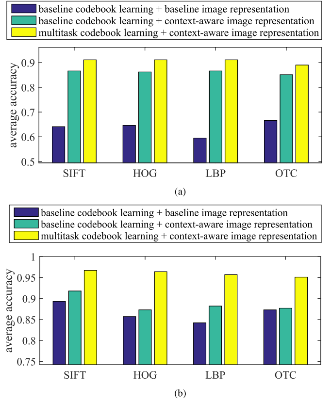
Fig. 11. Average scene classification accuracy of (1) baseline codebook learning + baseline image representation, (2) baseline codebook learning + context-aware image representation, and (3) multitask codebook learning + context-aware image representation. (a) MSRC dataset. (b) SIFT flow dataset.
