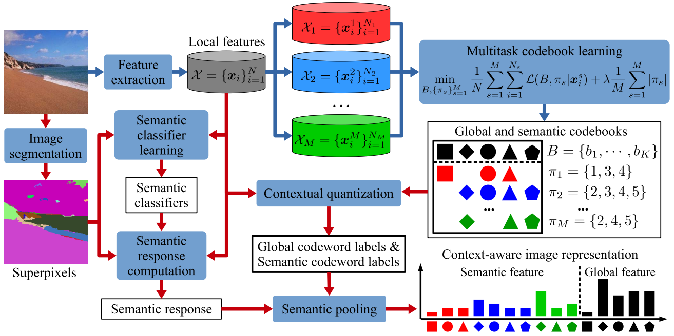
Fig. 2. The general framework of the proposed approach. The multitask semantic codebook learning is illustrated by the blue path. The context-aware image representation is illustrated by the red path.
