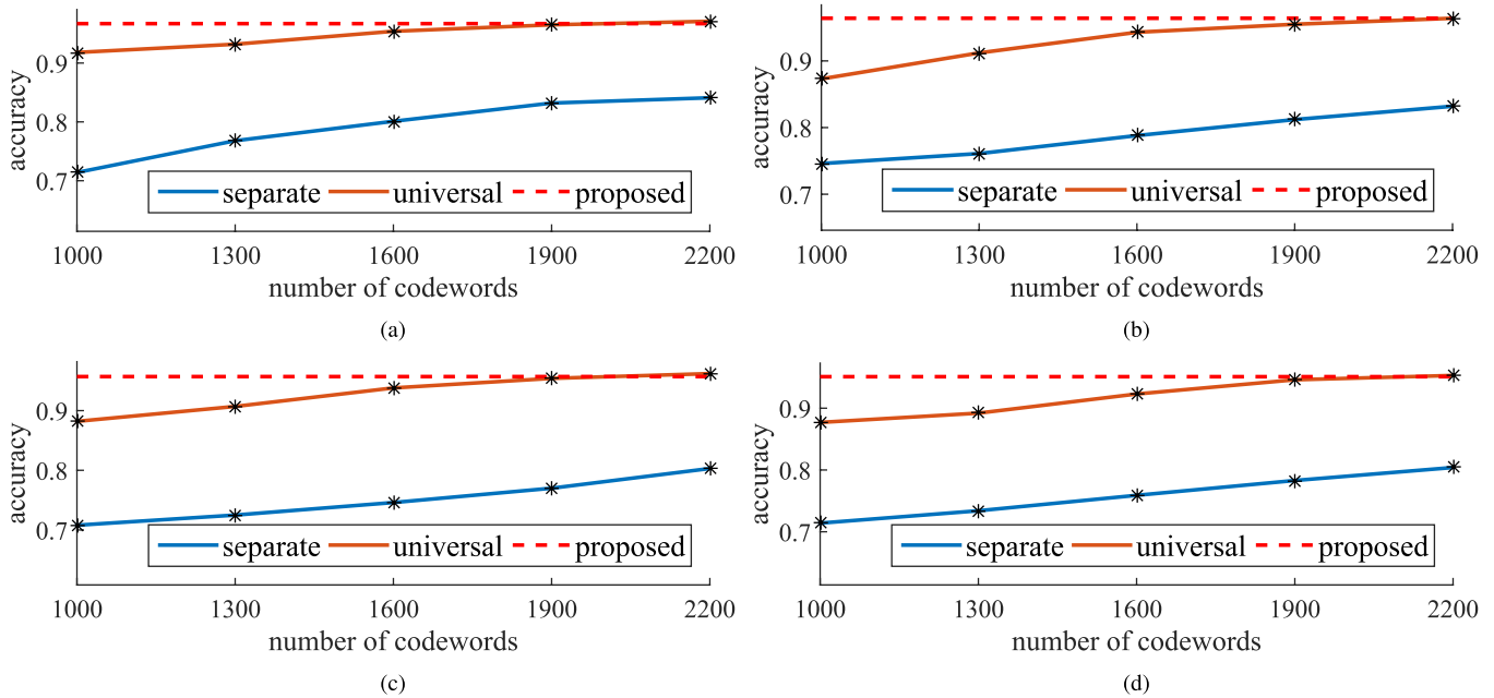
Fig. 8. Average scene classification accuracy of universal codebook learning and separate codebook learning with different number of codewords on the SIFT flow dataset. The performance of the proposed multitask codebook learning with 1000 codewords is illustrated with the dash line. (a) SIFT. (b) HOG. (c) LBP. (d) OTC.
