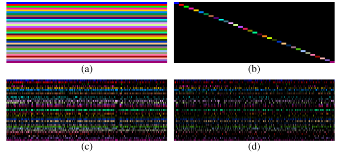
Fig. 13. Semantic codeword distribution of the universal codebook learning, the separate codebook learning and the multitask codebook learning on the SIFT flow dataset ( K = 1000, \lambda = 0.001, 0.005 ). Each column represents a global codeword, and each row represents a semantic class. Codewords selected by the semantic classes are marked in distinct colors, and the unselected ones are marked in black. (a) Universal codebook learning. (b) Separate codebook learning. (c) Multitask codebook learning ( \lambda = 0.001 ). (d) Multitask codebook learning ( \lambda = 0.005 ).
