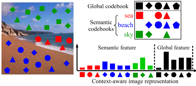
Fig. 1. The proposed method encodes the local features of each semantic class, e.g., beach , sea and sky , with a distinct semantic codebook, which is composed of a sparse subset of the global codebook, as illustrated in the top-right image. The image is represented in a context-aware manner by the distributions of the global and semantic codewords, as illustrated in the bottom-right image.
