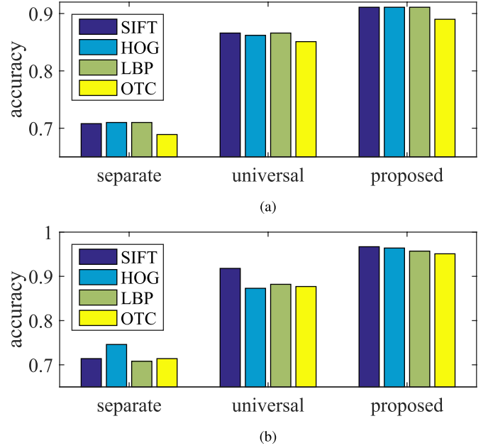
Fig. 6. Average scene classification accuracy of different codebook learning methods. (a) MSRC dataset ( K = 500 ). (b) SIFT flow dataset ( K = 1000 ).
