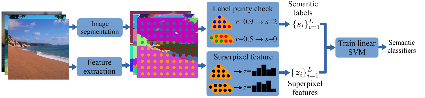
Fig. 4. Illustration of learning semantic classifiers. The input images are segmented into superpixels. The semantic label of a superpixel is determined by the label purity of the local features. The visual feature of each superpixel is encoded by the global codeword histogram. Finally, semantic classifiers can be obtained by learning linear SVM classifiers with the semantic labels and visual features of the superpixels.
