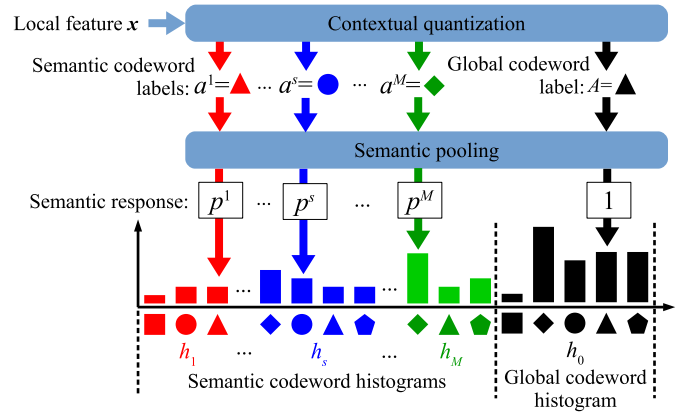
Fig. 3. The proposed context-aware image representation is computed via contextual quantization and semantic pooling. It contains both global and contextual distribution of codewords for representation.
