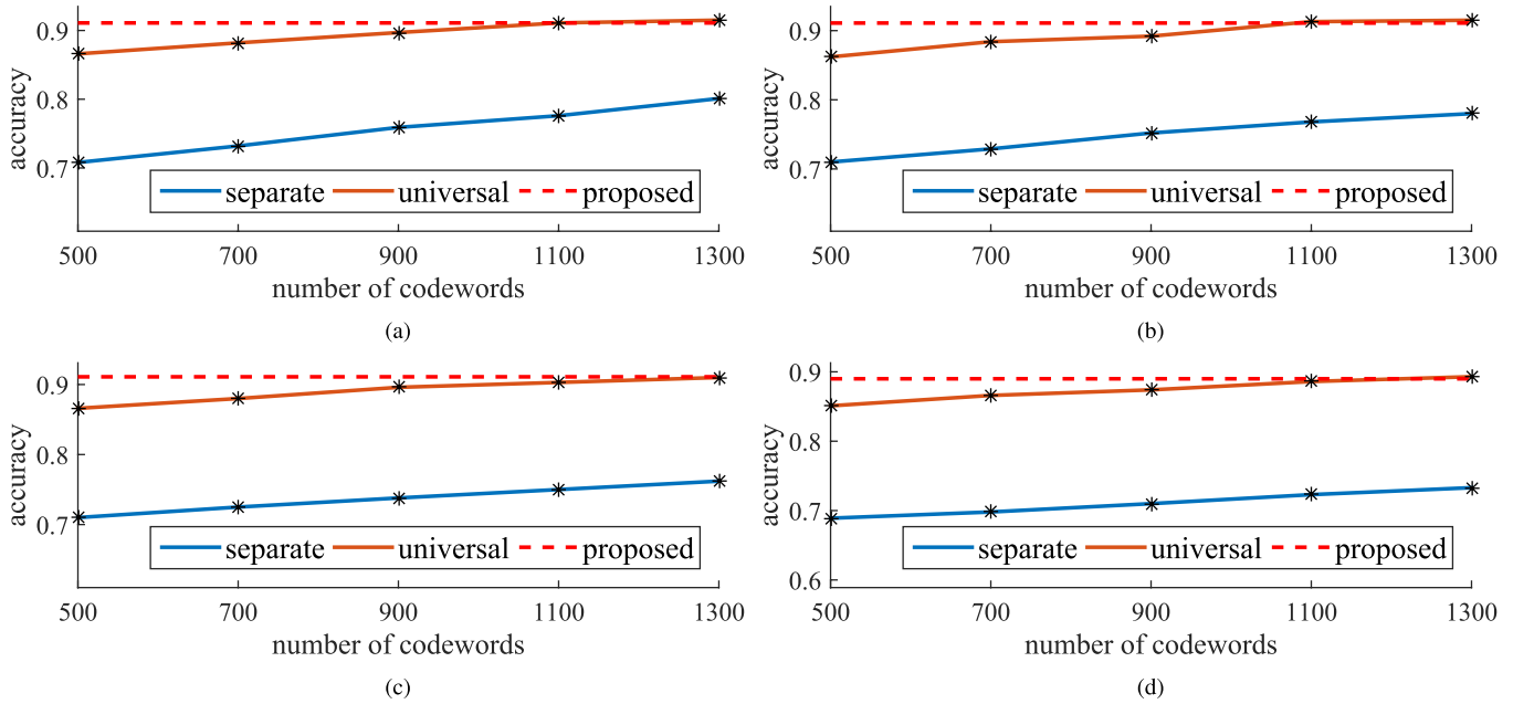
Fig. 7. Average scene classification accuracy of the universal codebook learning and the separate codebook learning with different number of codewords on the MSRC dataset. The performance of the proposed multitask codebook learning with 500 codewords is illustrated with the dash line. (a) SIFT. (b) HOG. (c) LBP. (d) OTC.
